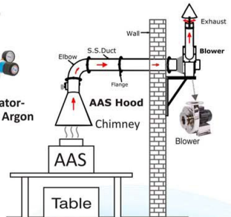
Fume Exhaust Hood
